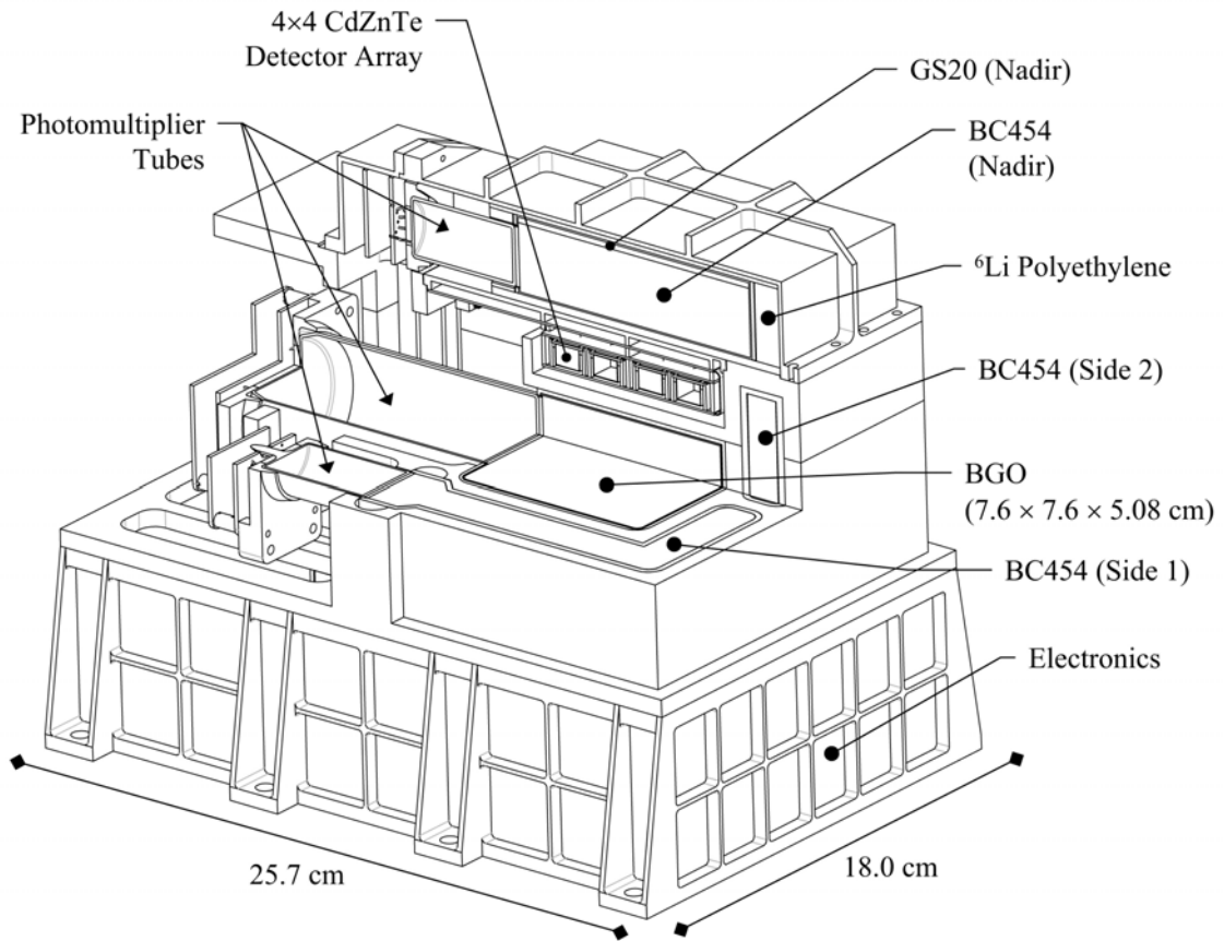
Fig.15 Gamma ray/neutron spectrometer
