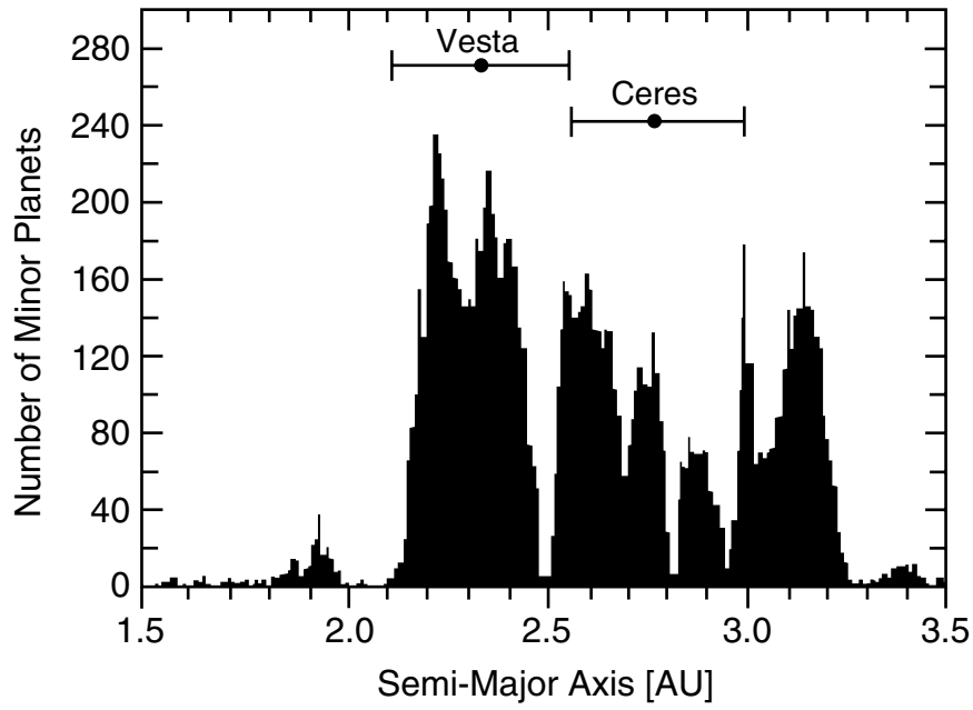
Fig 3 Number of asteroids versus semi-major axis in astronomical units with the range of heliocentric distances over which Vesta and Ceres travel
