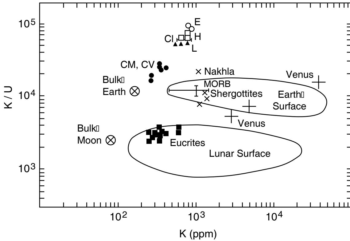
Fig.14 Potassium to uranium ratio versus potassium concentration [Taylor, 1992]
