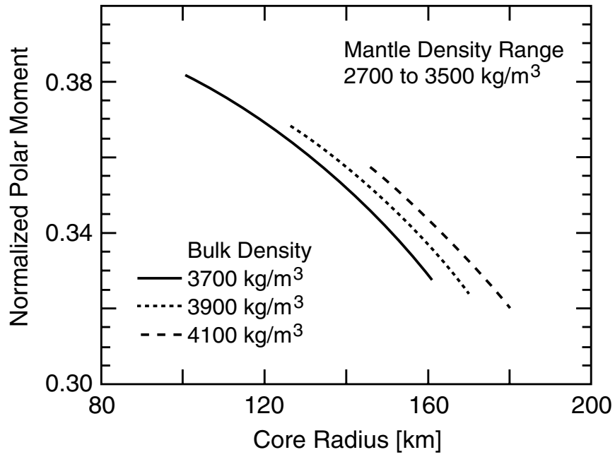
Fig.19 Polar moment of inertia versus core radius of Vesta
