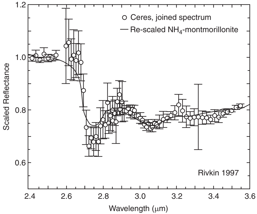
Fig.12 Spectrum of Ceres illustrating absorption near 3\mu\text{m} [Rivkin 1997]
