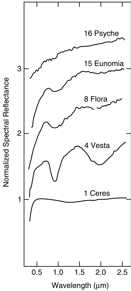
Fig.11 Normalized reflectance spectra of major asteroids [Gaffey et al., 1989]
